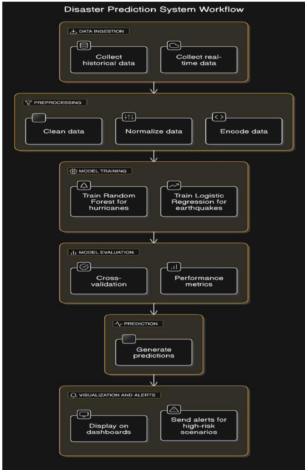
Figure 4.1: workflow chart
